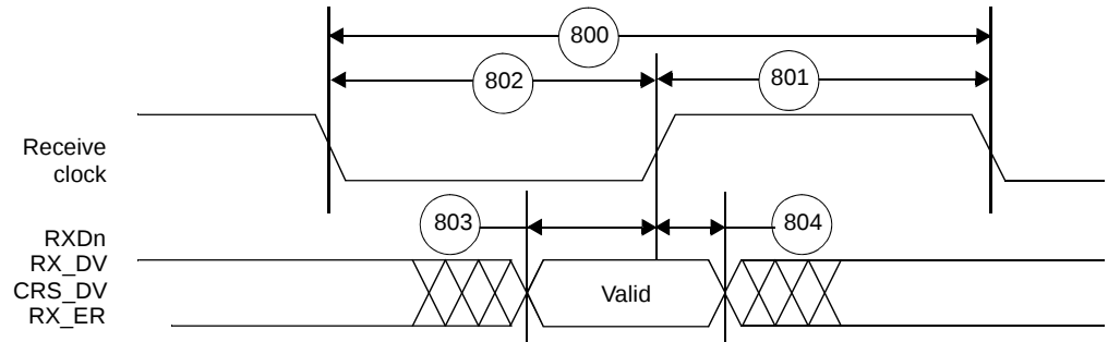
Figure 10. Ethernet Receive Signal Timing
